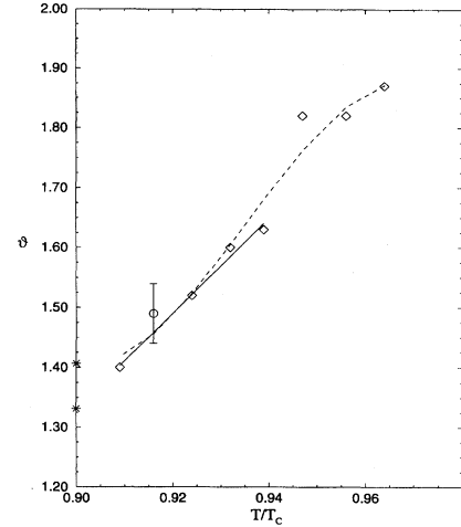
FIG. 1. A cubic fit of the simulation results for \theta(T, \dots) . A linear fit to the lower four diamonds is also shown. The extrapolated values \theta^+ at T_W/T_C \sim 0.9 are indicated by stars. Apart from the data point at T/T_C = 0.916 the error is within the symbol. As the temperature rises from T_W the value of \theta increases.
